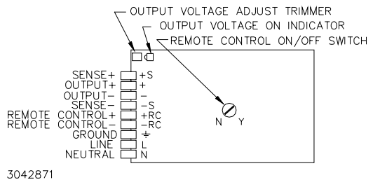
FIGURE 2. COMPONENT LOCATIONS
